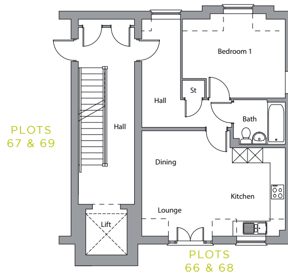
OXFORD SPECIAL (FIRST & SECOND FLOOR)
